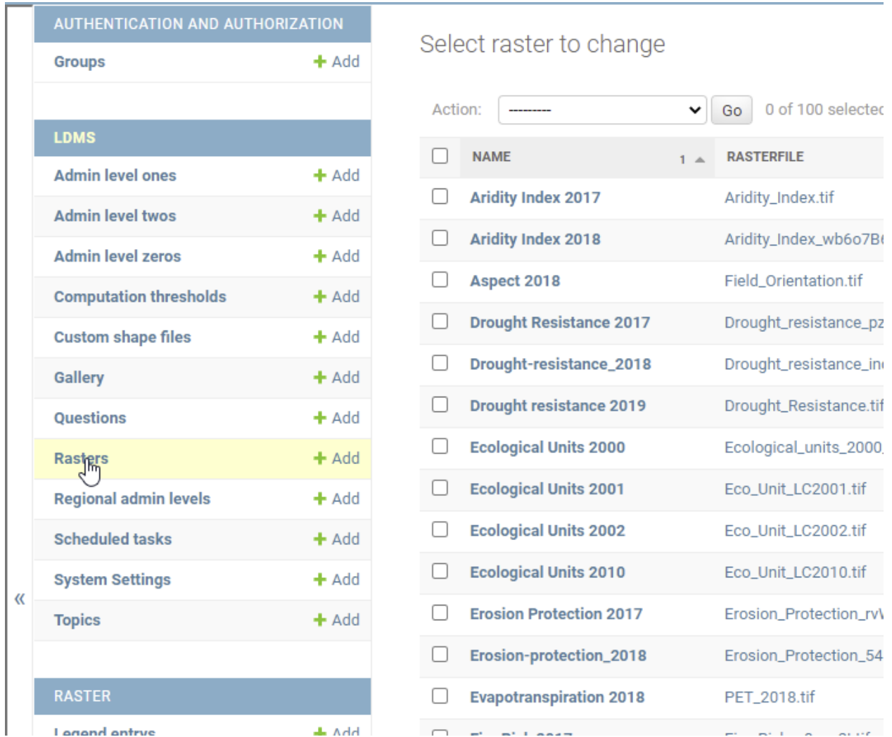
Fig. 8: Uploading rasters
