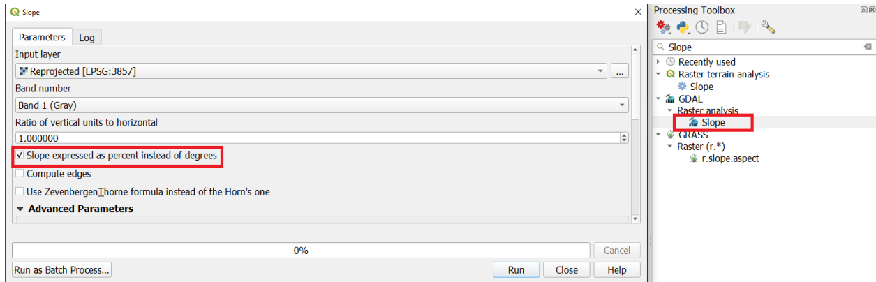
Fig. 6: Slope Computation
