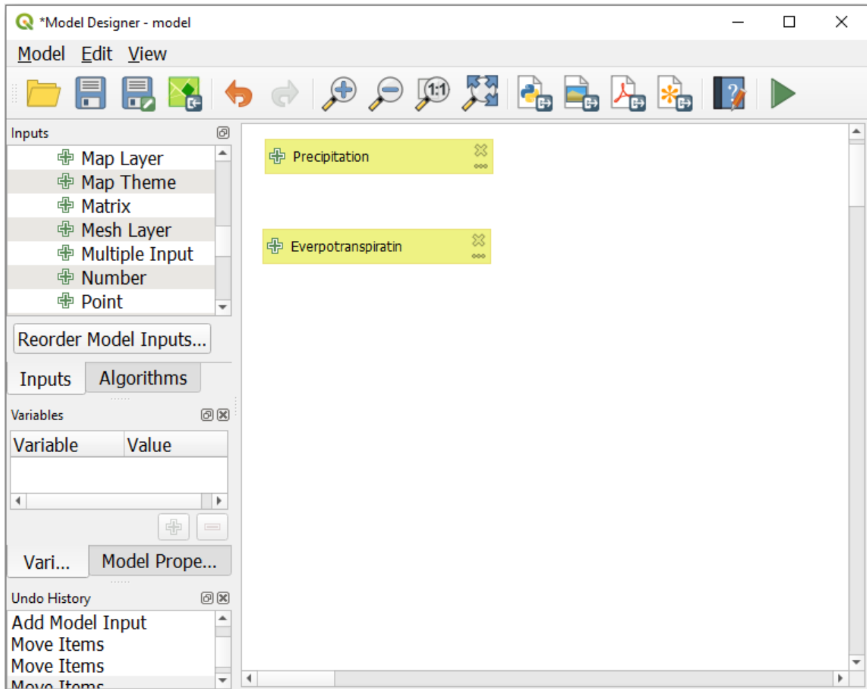
Fig. 4: Model Inputs
